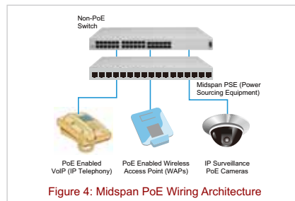
Figure 4: Midspan PoE Wiring Architecture
